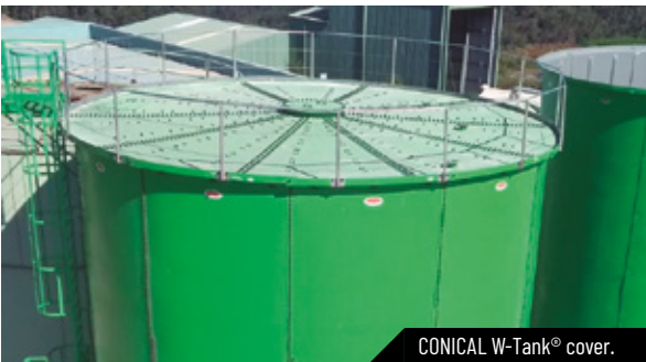
FLAT W-Tank® hermetic cover for digesters
