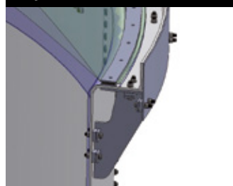
Fastening system for gasometer and membranes
