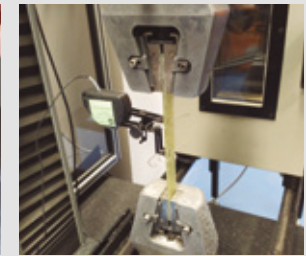
Traction test
